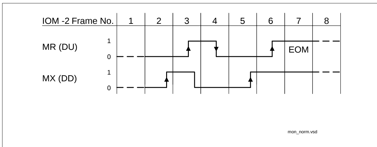
Figure 35 Monitor Channel, normal End of Transmission
