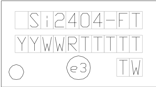
Figure 17. Si2404-D-FT Top Marking
