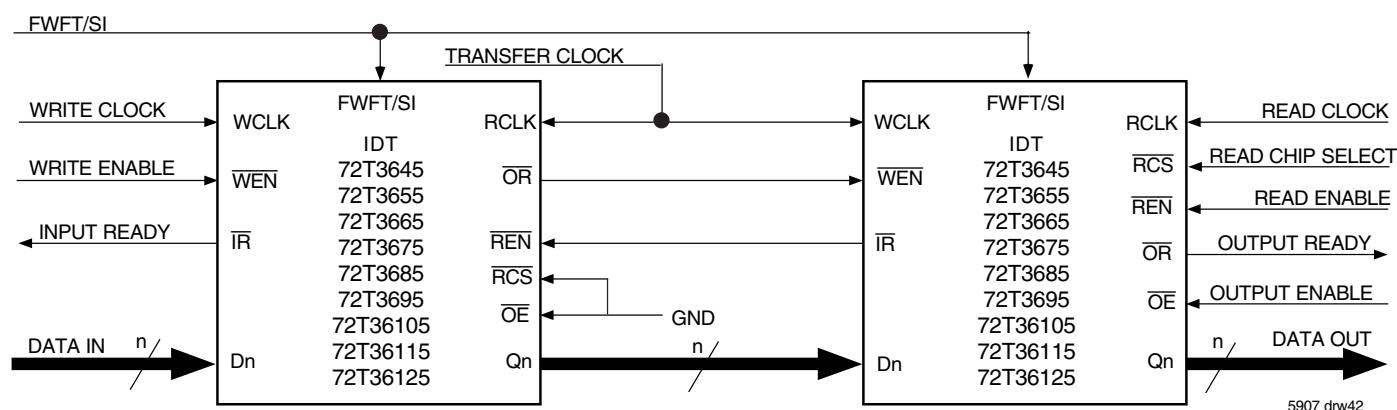
Figure 37. Block Diagram of 2,048 x 36, 4,096 x 36, 8,192 x 36, 16,384 x 36, 32,768 x 36, 65,536 x 36, 131,072 x 36, 262,144 x 36 and 524,288 x 36
