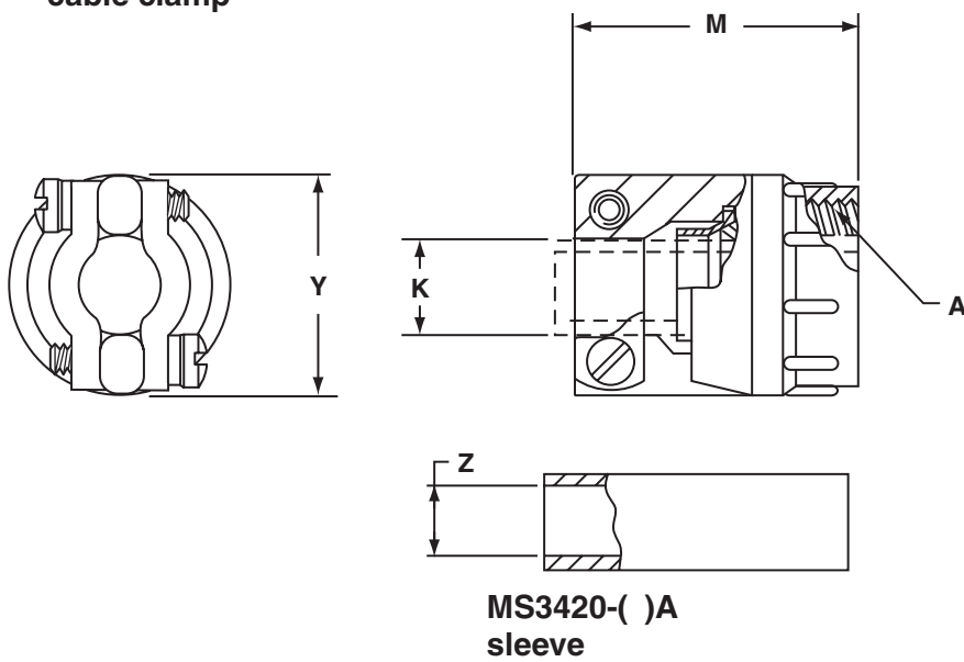
10-350349-( )3 cable clamp
