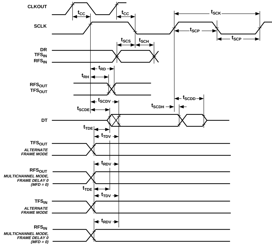
Figure 13. Serial Ports
