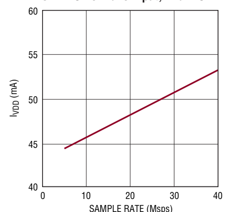
LTC2264-14: I_{VDD} vs Sample Rate, 5\text{MHz} Sine Wave Input, -1\text{dBFS}
