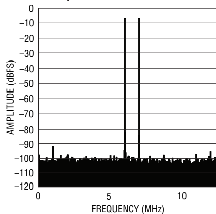
LTC2263-14: 8k Point 2-Tone FFT, f_{IN} = 68\text{MHz} , 69\text{MHz} , -1\text{dBFS} , 25Msps
