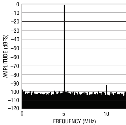
LTC2263-14: 8k Point FFT, f_{IN} = 5\text{MHz} , -1\text{dBFS} , 25Msps
