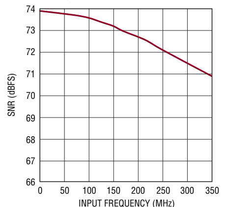
LTC2265-14: SNR vs Input Frequency, -1\text{dBFS} , 2\text{V} Range, 65\text{Mps}
