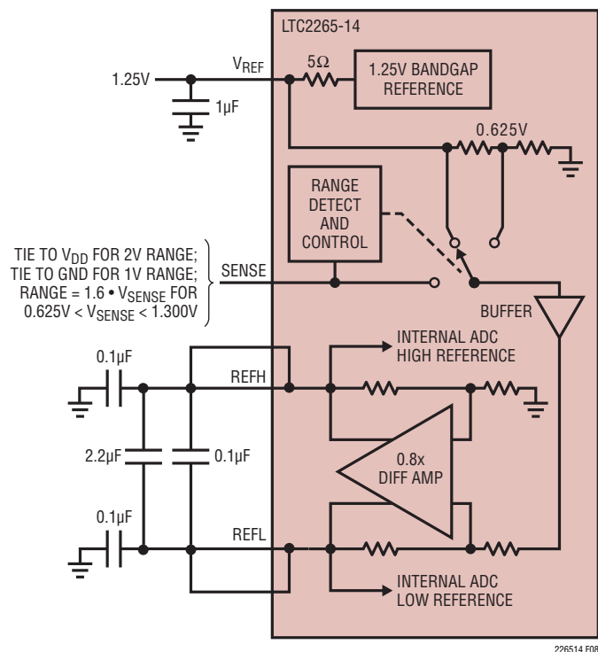
Figure 8. Reference Circuit
