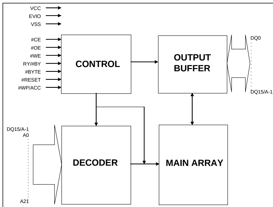
Figure 4-1 Block Diagram
