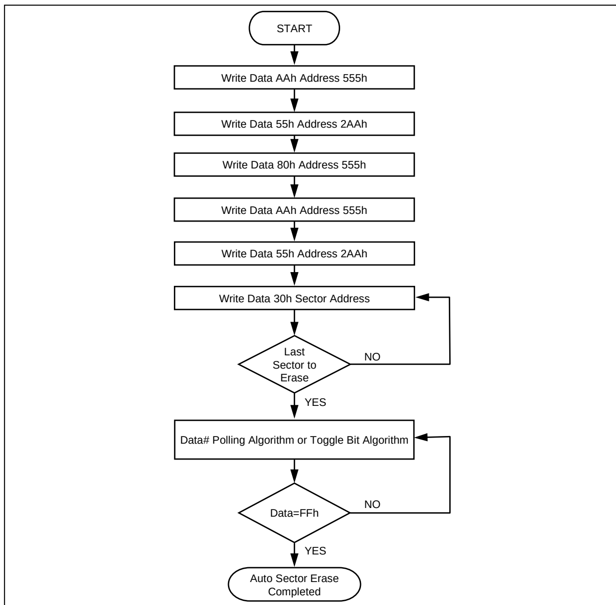
Figure 8-11 Automatic Sector Erase Algorithm Flowchart
