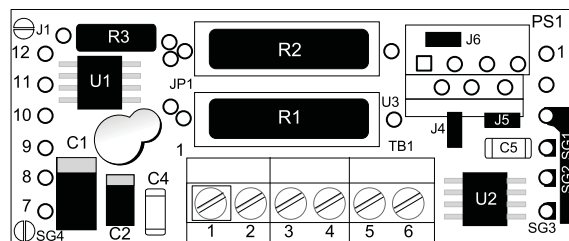
Figure 2. DMS-EB-RMS Board
