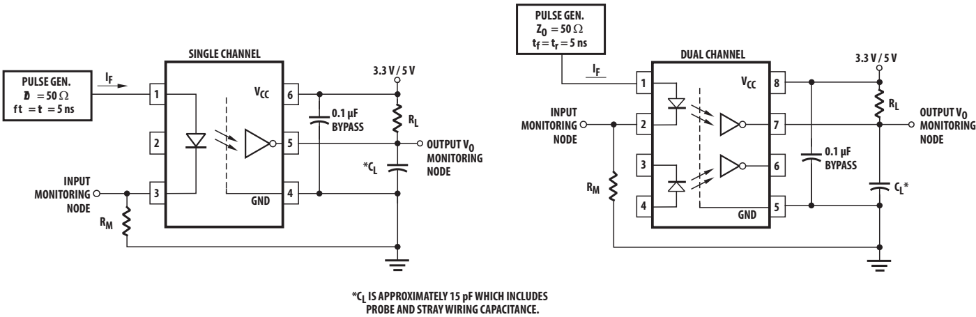
Figure 10 Test Circuit for t_{pHL} and t_{pLH}
