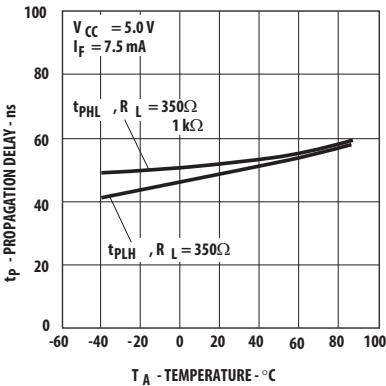
Figure 12 Typical Propagation Delay vs. Temperature V_{CC} = 5V
