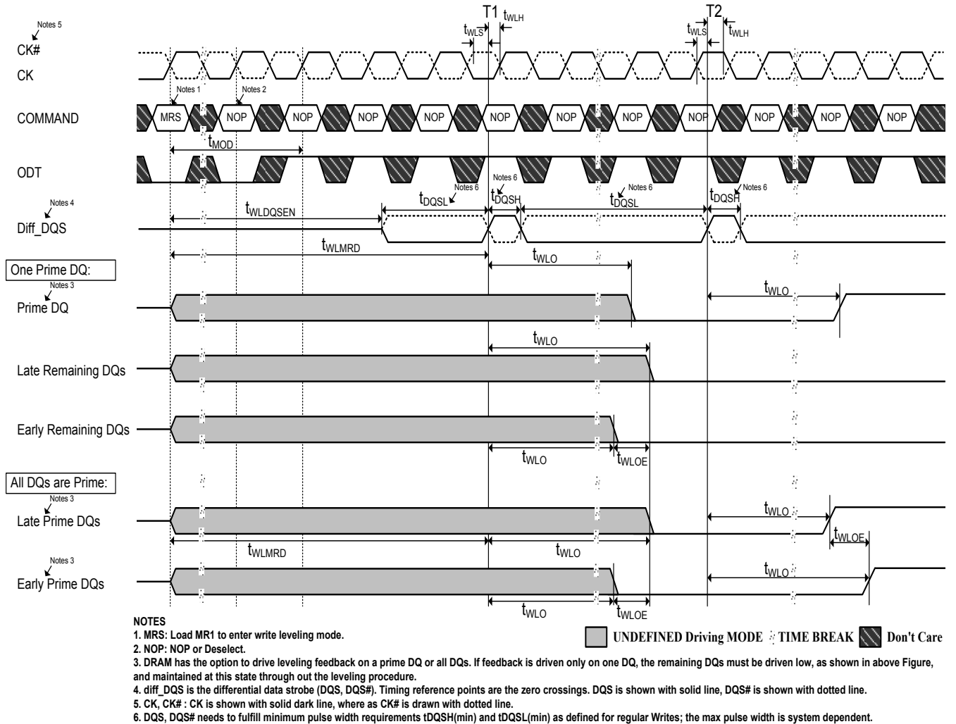
Figure14. Timing details of Write Leveling sequence (DQS – DQS# is capturing CK – CK# low at T1 and CK – CK# high at T2)
