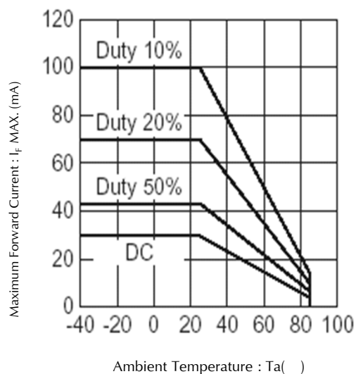
Ambient Temperature vs. Maximum Forward Current f = 50Hz
