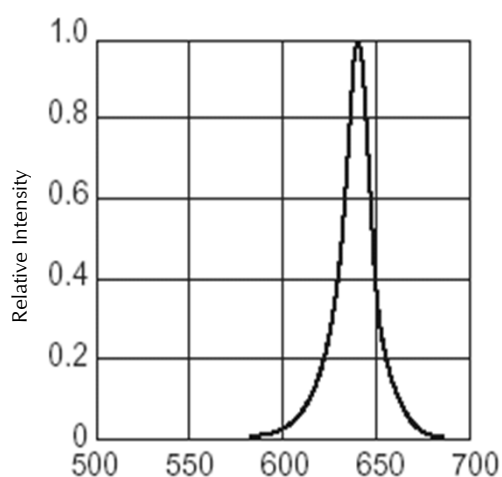
Relative Intensity vs. Wavelength Condition : T_a = 25 , I_F = 20\text{mA}
