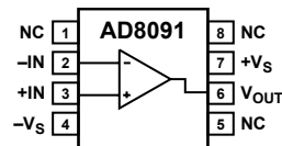
Figure 1. SOIC-8 (R-8)
