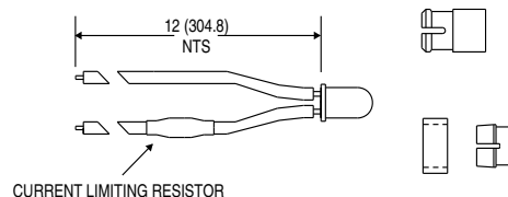
PH25 Outline
