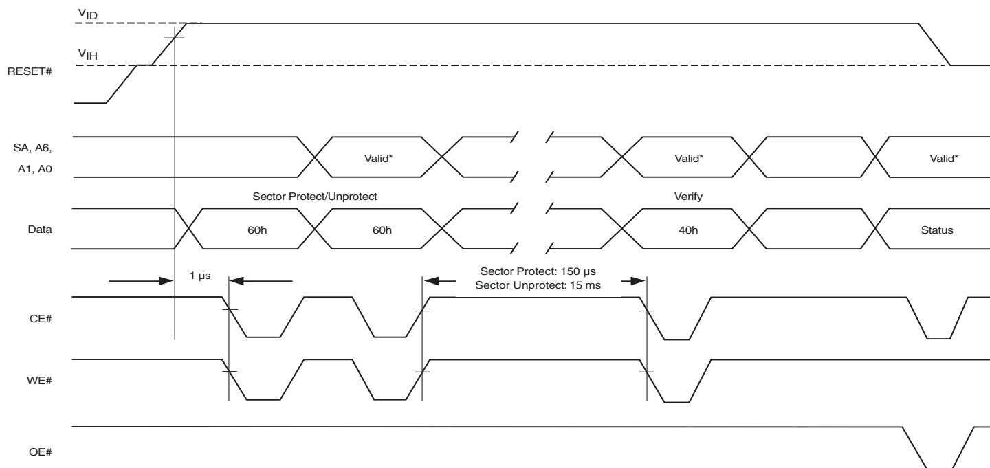
Figure 13.12 Sector Protect/Unprotect Timing Diagram
