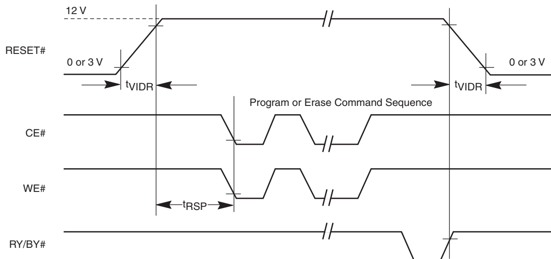
Figure 10-11 Temporary Sector Unprotect Timing Diagram
