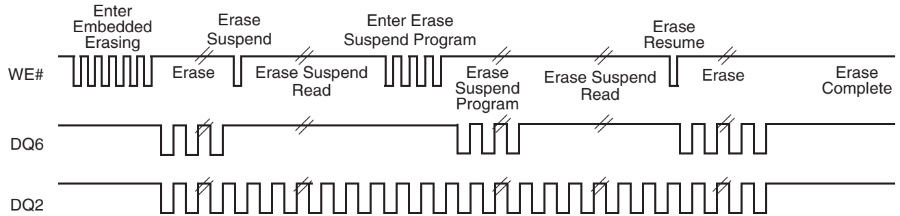
Figure 10-10 DQ2 vs. DQ6
