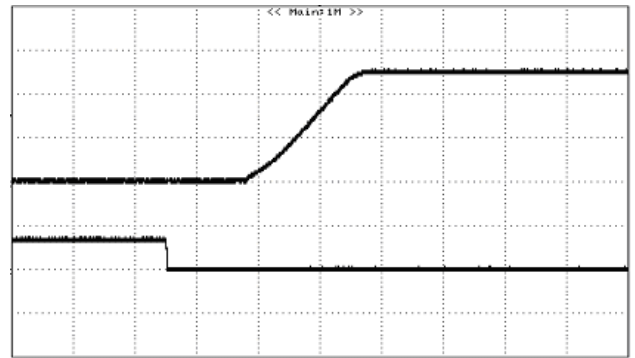
Figure 14: Turn on Using Remote On/Off with external capacitors ( C_o= 3000 \mu F ), 5.0V/5A out (resistive load)(10mS/div)
