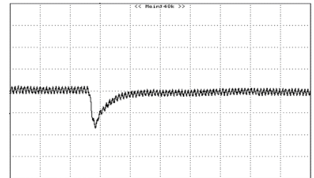
Figure 16: Typical transient response to step load change at 2.5A/μS from 50% to 100% of I_o , max at 12Vin, 5.0V out ( C_{out} = 1\mu F ceramic+ 10μF Ceramic)(100mV/div, 20uS/div)
