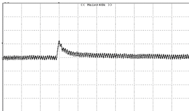
Figure 15: Typical transient response to step load change at 5A/μS from 100% to 50% of I_o , max at 12Vin, 5.0V out ( C_{out} = 1\mu F ceramic+ 47μF Ceramic)(100mV/div, 20uS/div)
