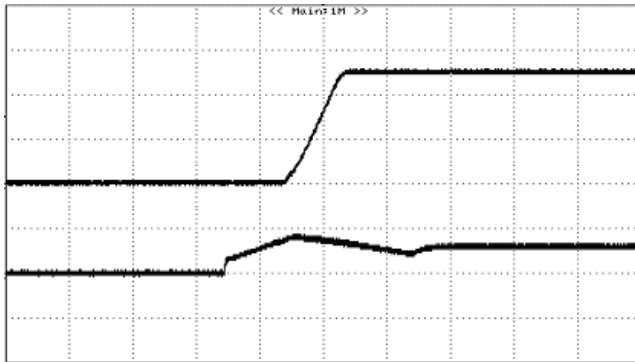
Figure 13: Turn on Using Input On/Off with external capacitors ( C_o=3000 \mu F ), 5.0V/5A out (resistive load)(10mS/div)
