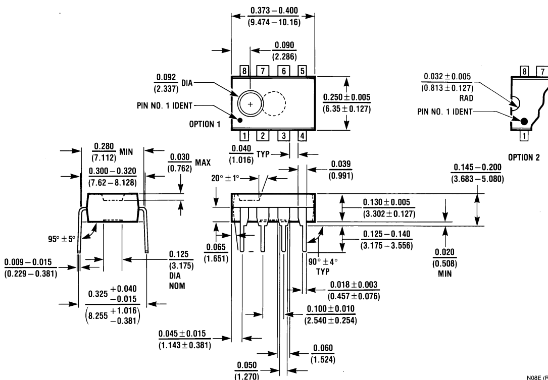
8-Lead (0.300" Wide) Molded Dual-In-Line Package Order Number LM4862N NS Package Number N08E
