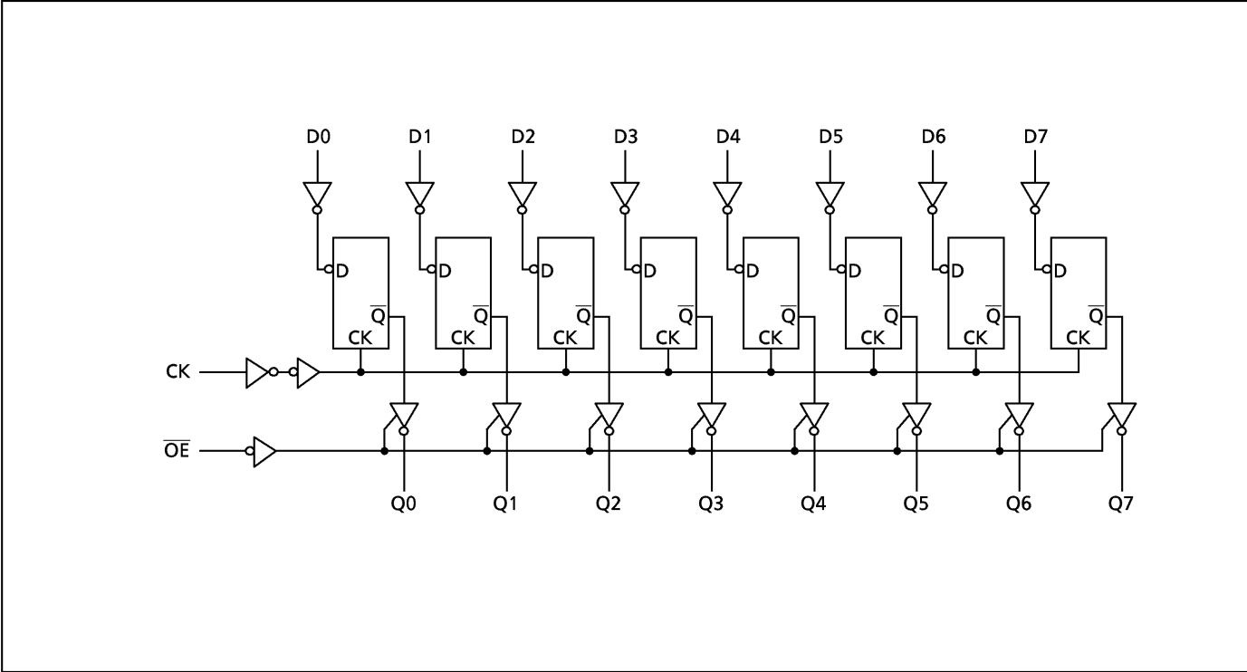
SYSTEM DIAGRAM
