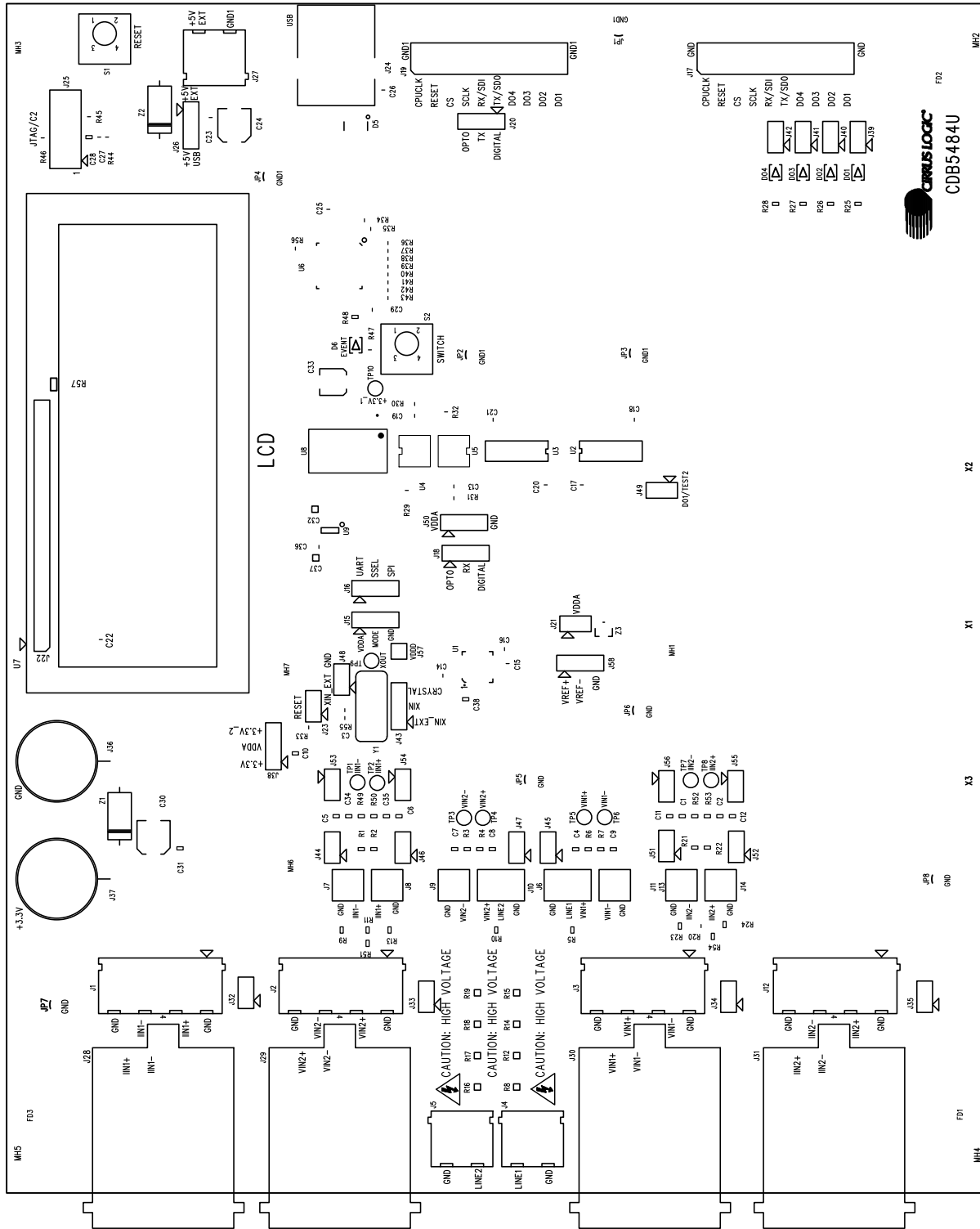
Figure 36. Top Silkscreen
