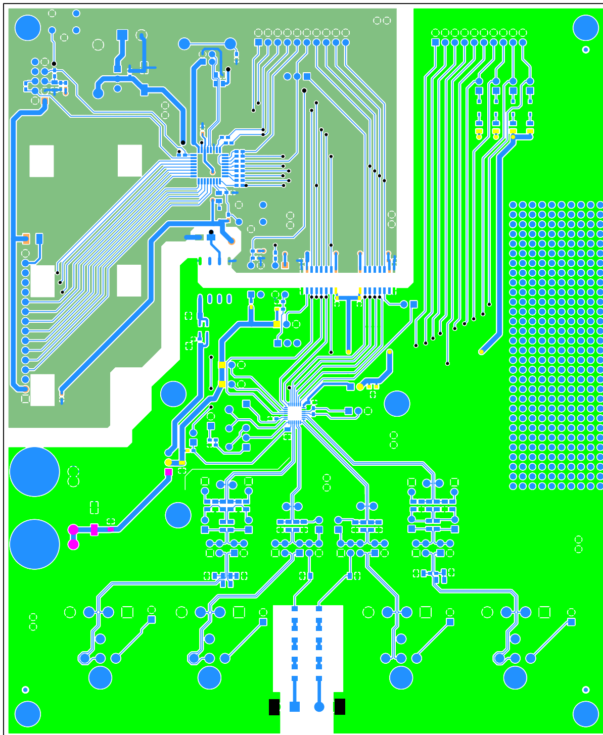
Figure 37. Top Routing
