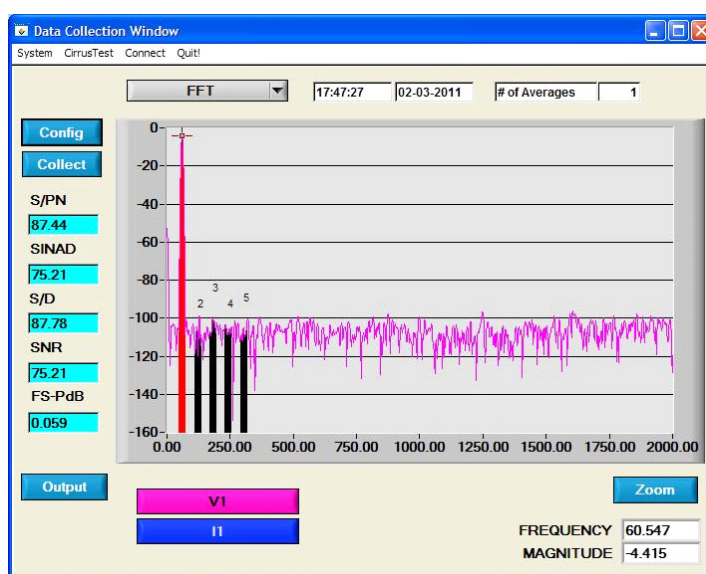
Figure 27. FFT Analysis
