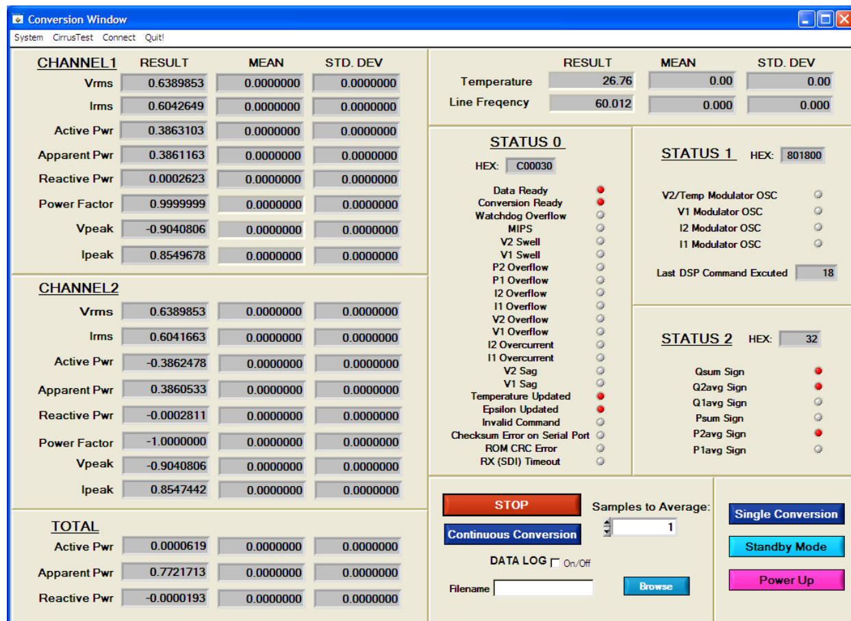
Figure 20. Conversion Window
