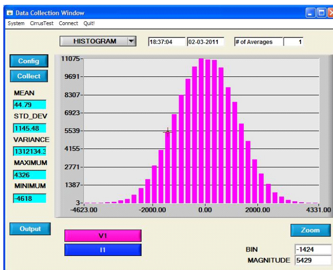
Figure 26. Histogram Analysis
