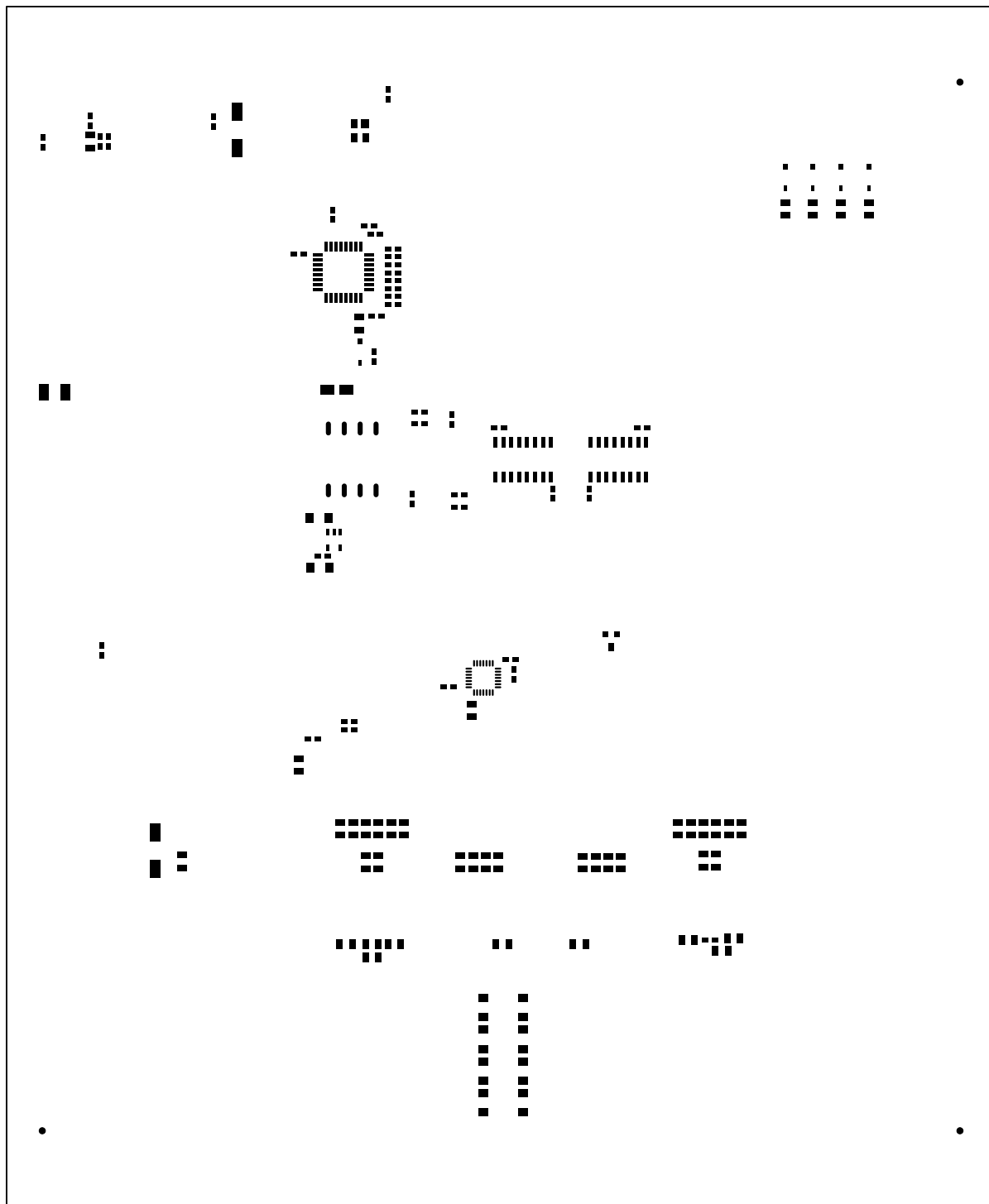
Figure 39. Solder Paste Mask
