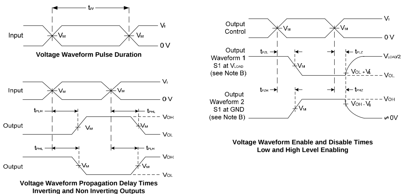
Figure 1 Load Circuit and Voltage Waveforms
