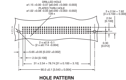
HOLE PATTERN
