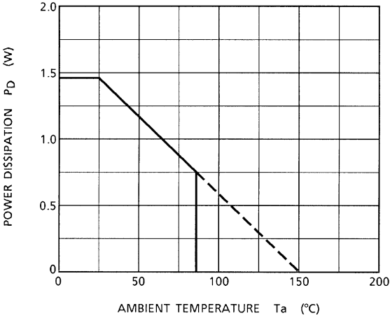
P_D - T_a
