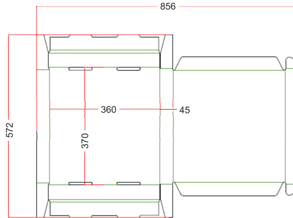
Figure 12-4. Reel Box
