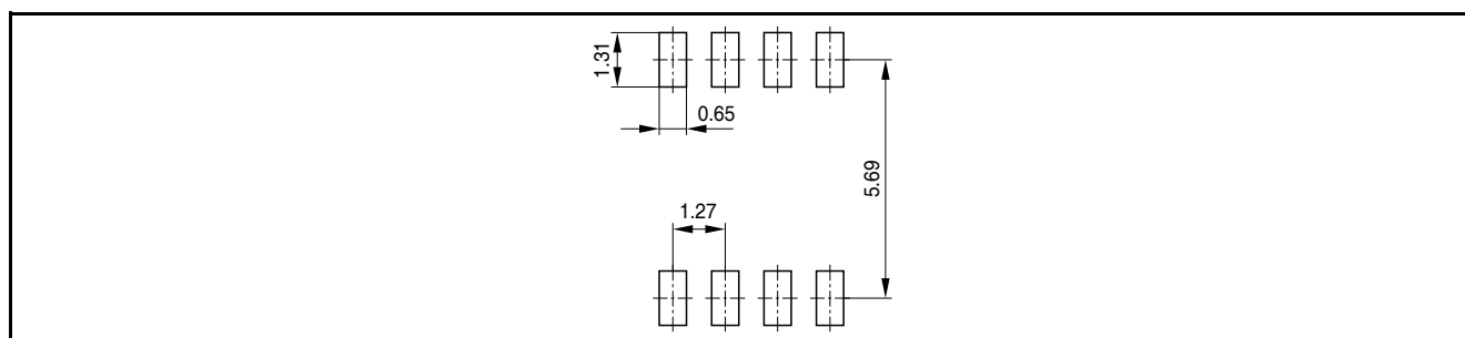
Figure 10 Footprint PG-DSO-8
