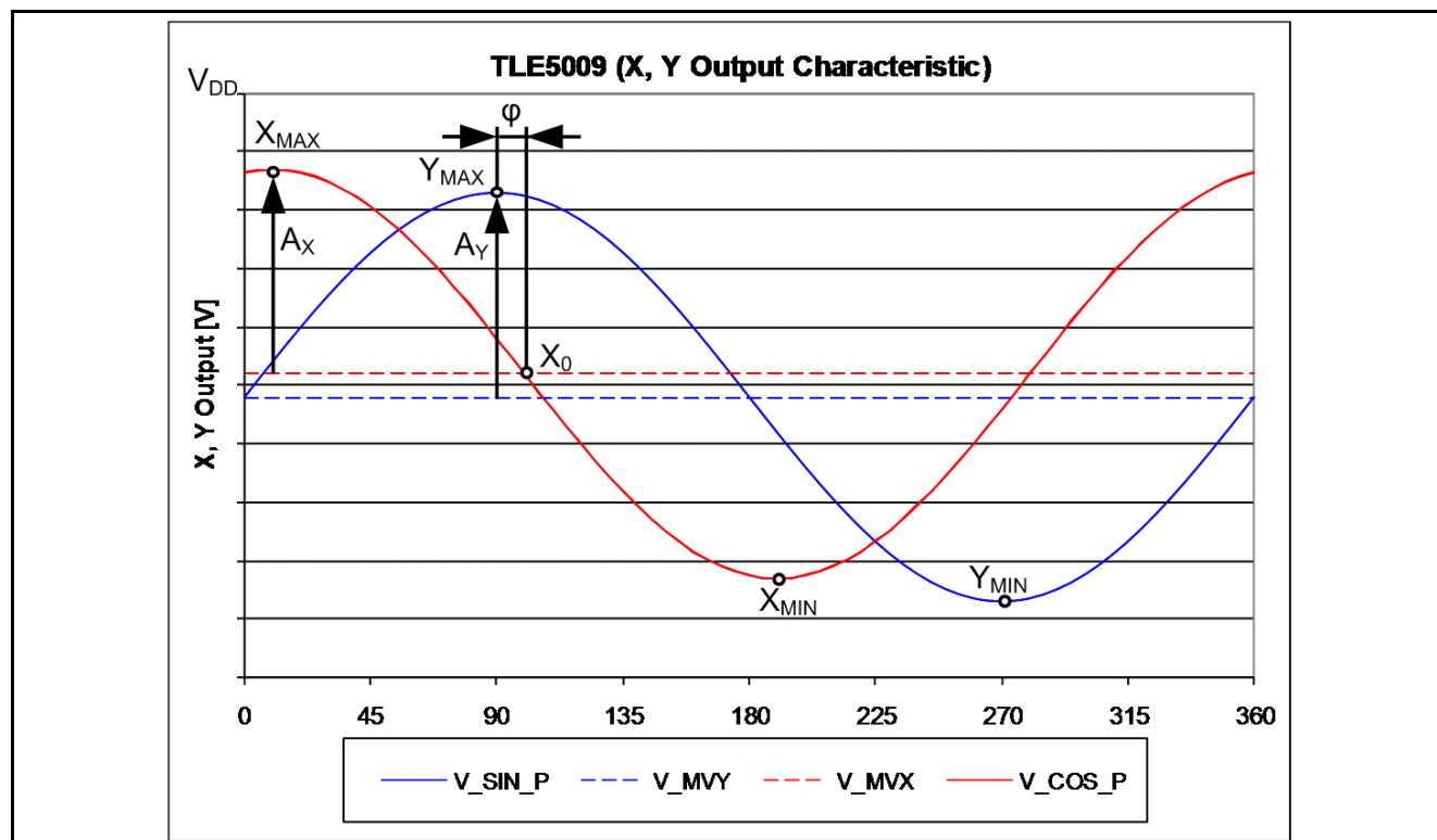
Figure 6 Single ended output signals
