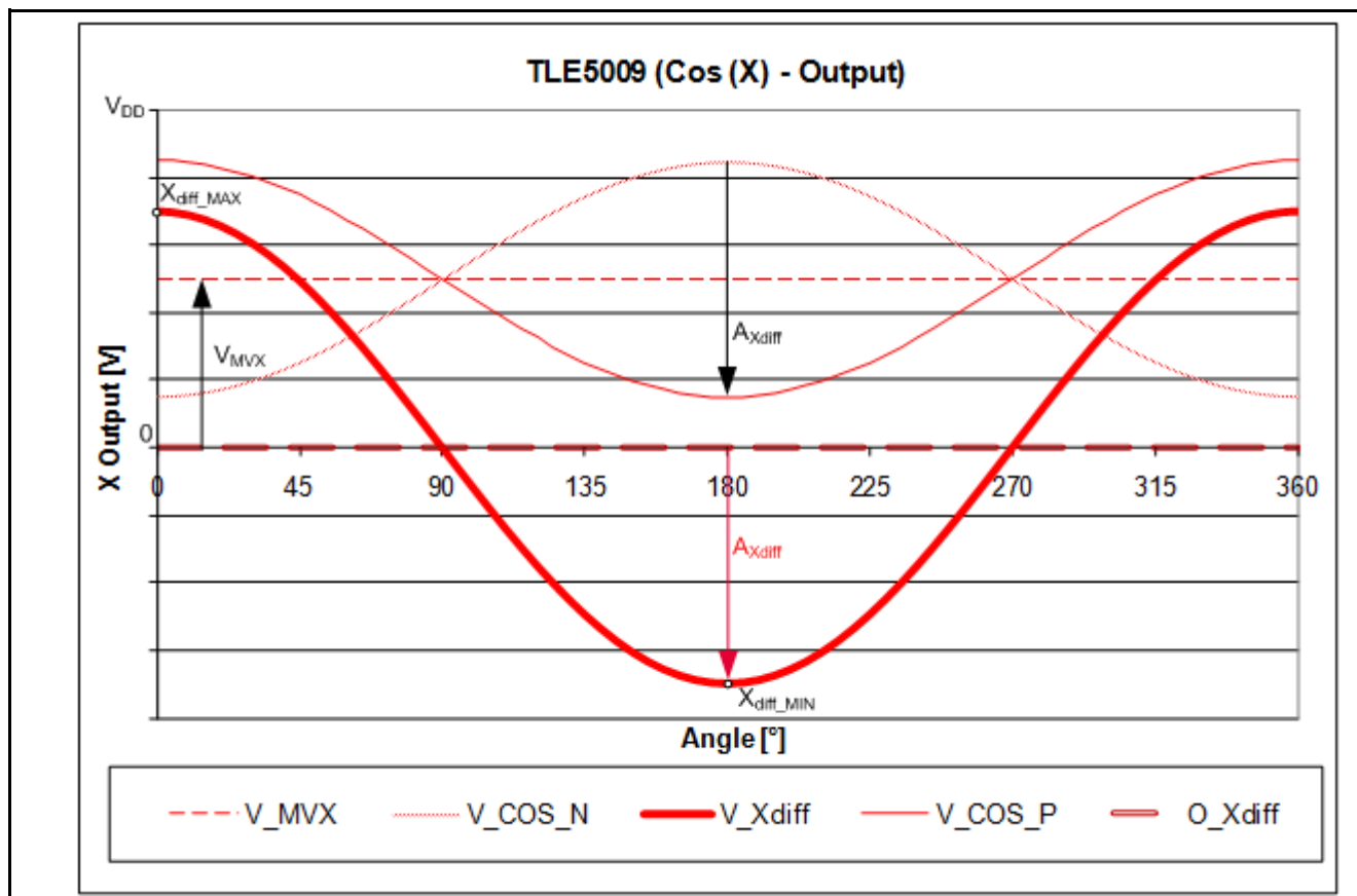
Figure 7 Differential output of ideal cosine
