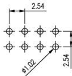
Recommended P.C.Board Hole Layout
