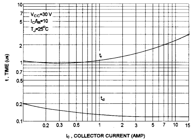
TURN-ON TIME
