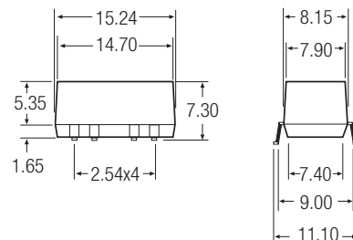
6 PIN Dual SMD Package
