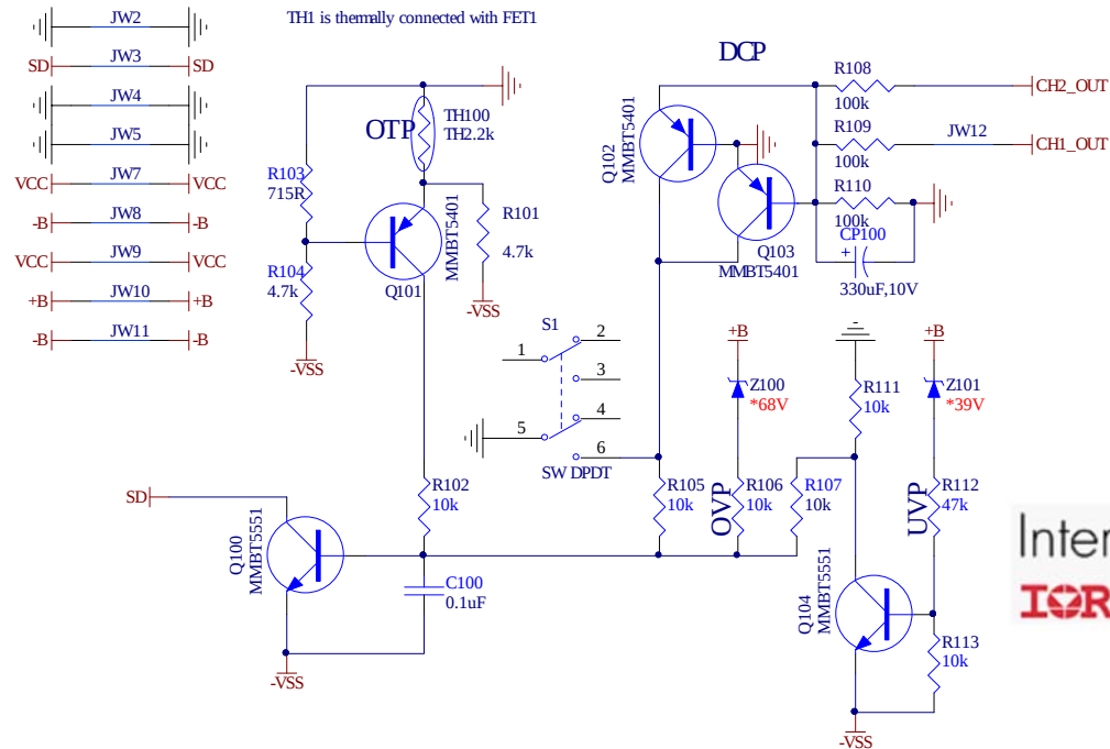
Fig 34 Protection Schematic
