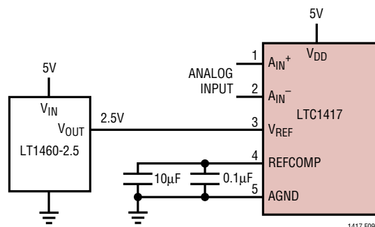
Figure 9. Using the LT1460 as an External Reference
