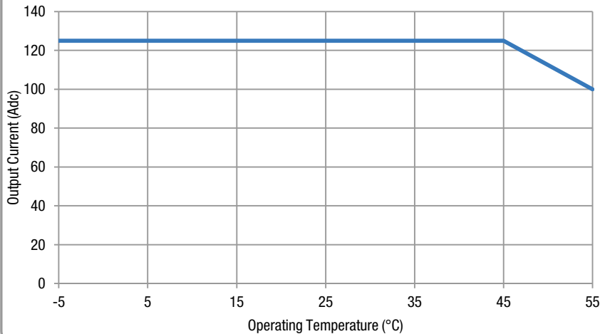
D1U54-D-1500-12-HxxPC Derating With Temperature
