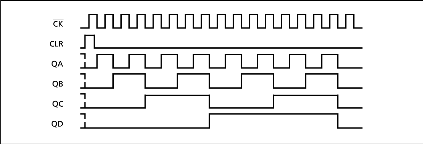
TIMING CHART
