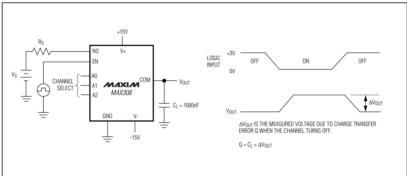
Figure 5. Charge Injection
