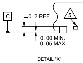
DETAIL "X"
