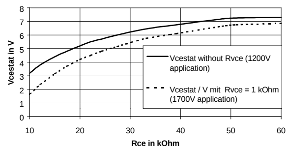
Fig. 4 V_{CEstat} in dependence of R_{CE}
