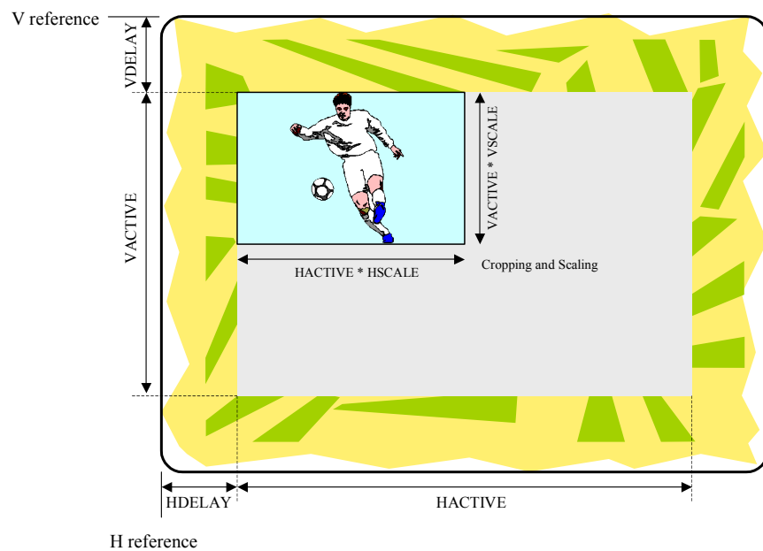
Fig 10 The Effect of Cropping and Scaling Active Registers
