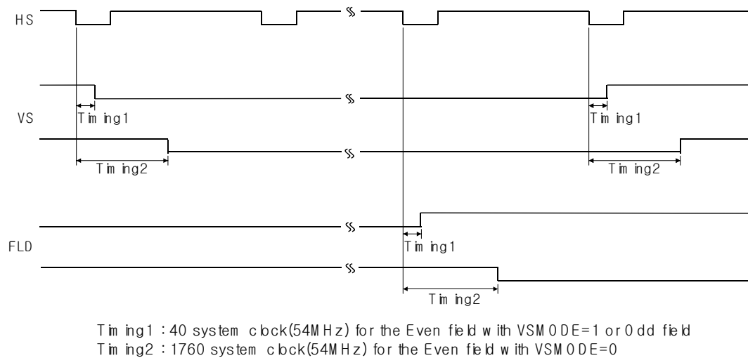
Fig 14 Horizontal and Vertical Timing in Video Output
