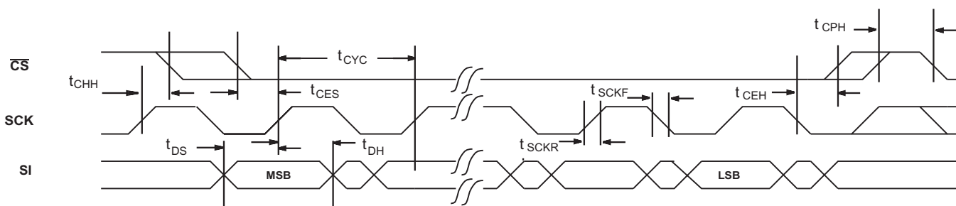
FIGURE 12. SPI Serial Input Timing
