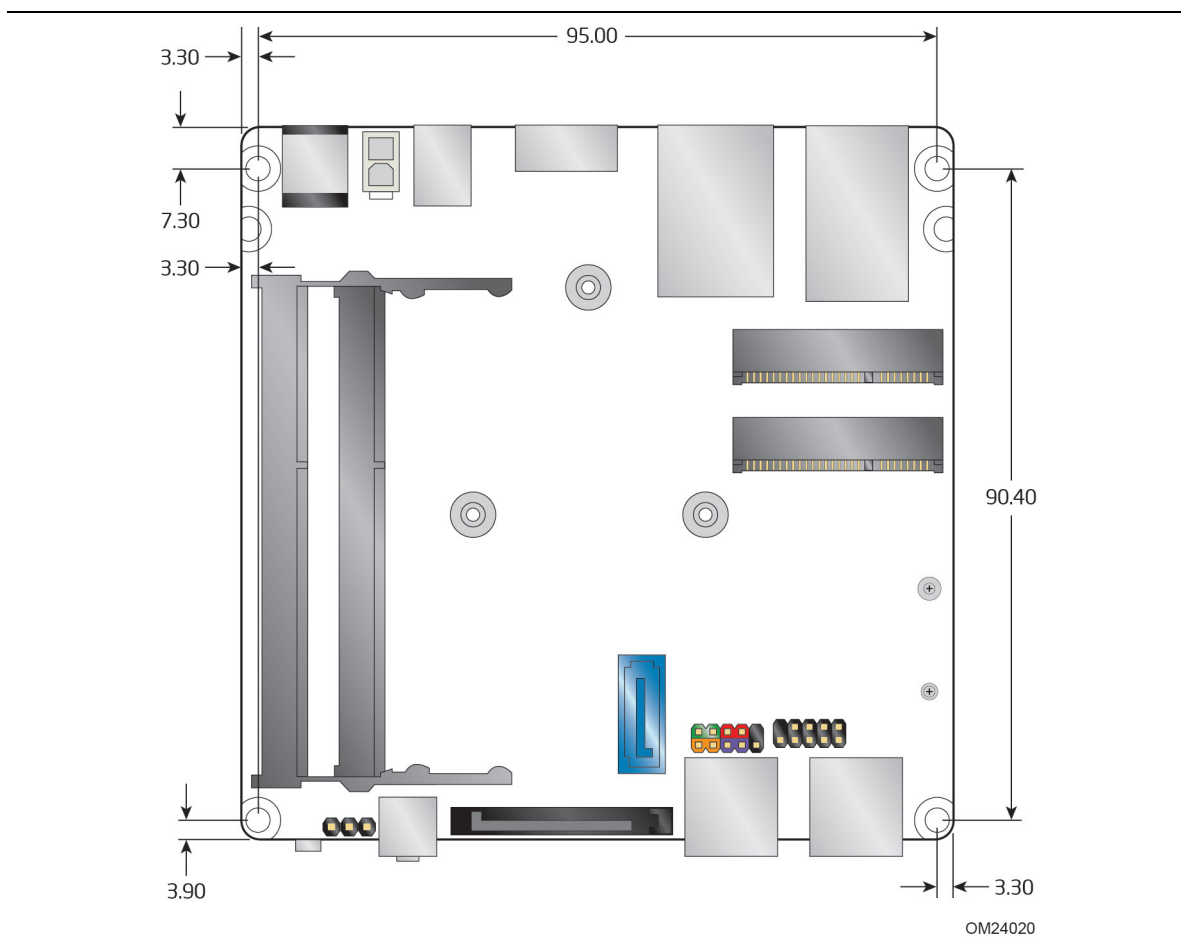
Figure 17. Board Dimensions
