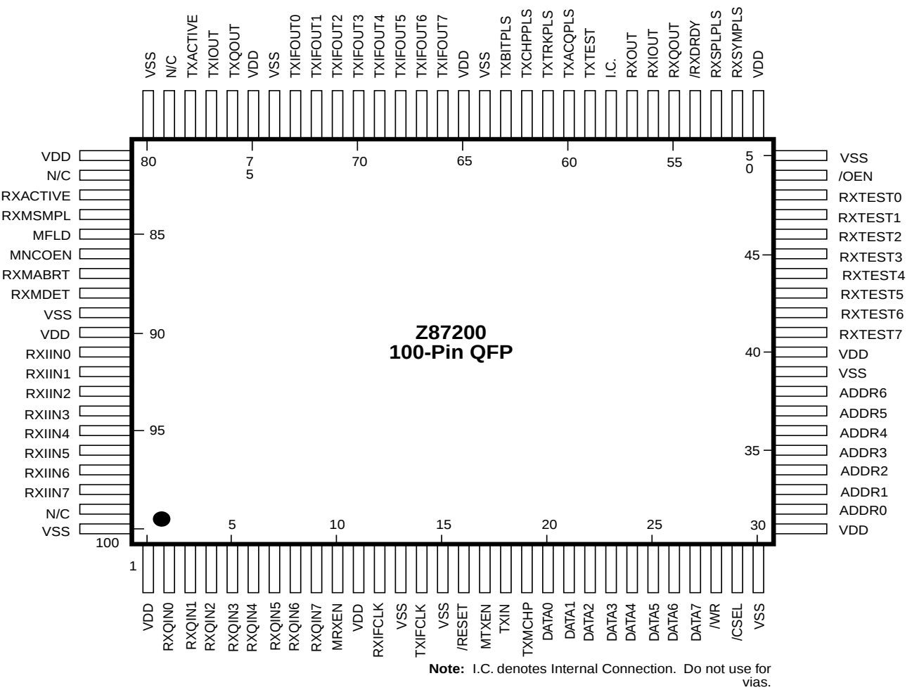
Figure 2. Z87200 100-Pin PQFP Pin Description
