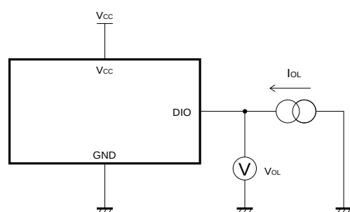
Fig.1 LOW output voltage measurement circuit
