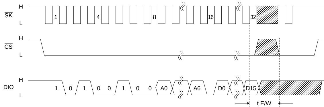
Fig.15 Data write
