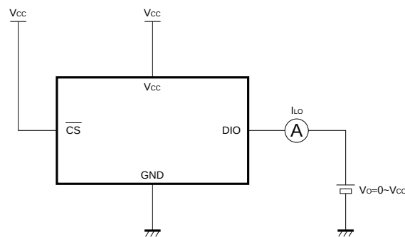
Fig.4 Output leakage current measurement circuit
