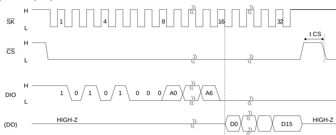
Fig.14 Data read
