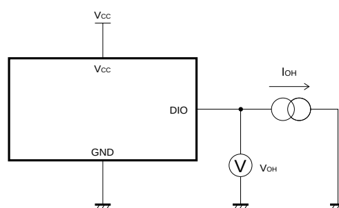
Fig.2 HIGH output voltage measurement circuit
