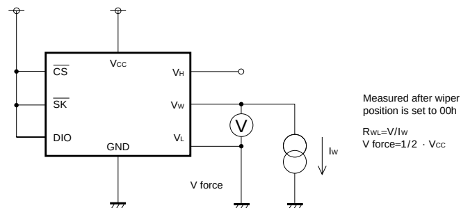
Fig.8 Wiper resistance measurement circuit on Low side
