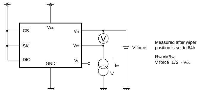
Fig.9 Wiper resistance measurement circuit on High side
