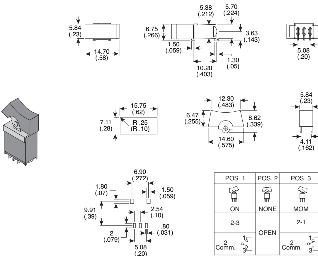
P.C. MOUNTING
