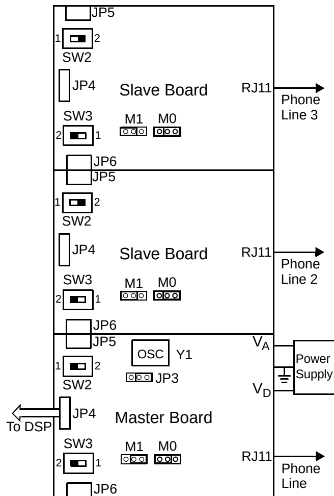
Figure 2. Daisy-Chain Connections
