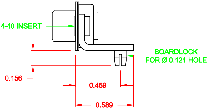
MOUNTING HARDWARE
