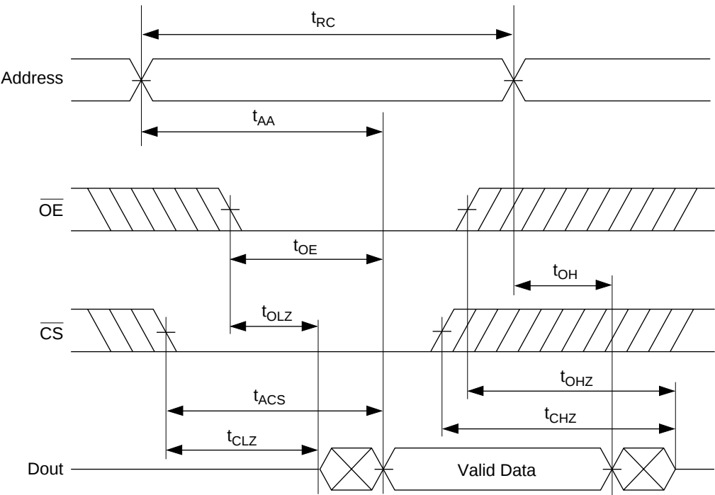
Read Cycle Timing-1*1 ( \overline{WE} = V_{IH} )
