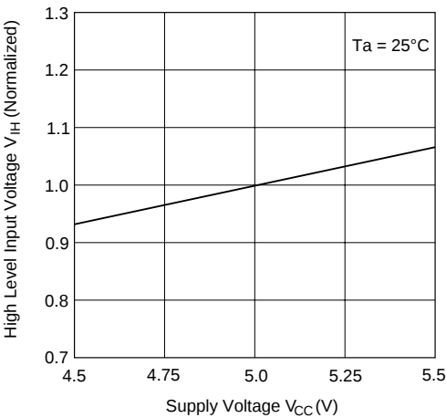
High Level Input Voltage vs. Supply Voltage
