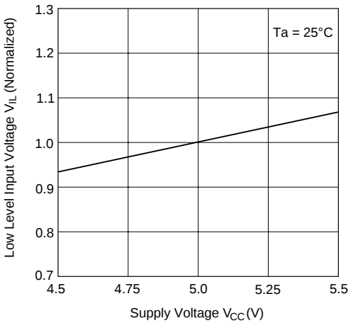
Low Level Input Voltage vs. Supply Voltage
