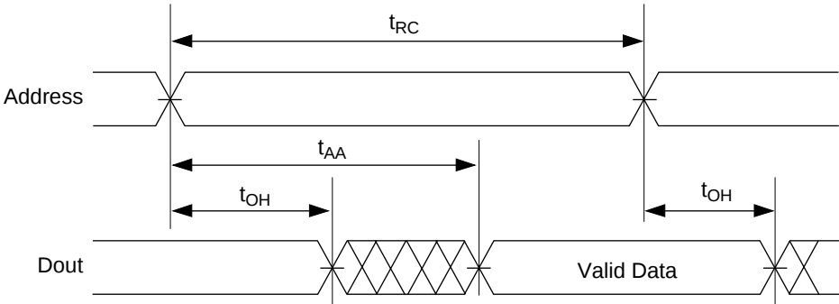
Read Cycle Timing-2 ( \overline{WE} = V_{IH} , \overline{CS} = V_{IL} , \overline{OE} = V_{IL} )
