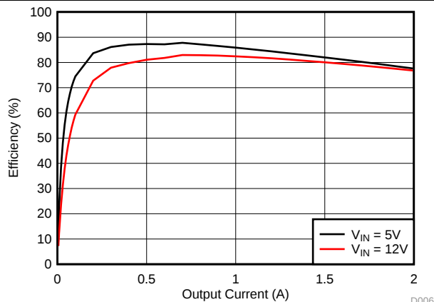
Figure 18. TPS562219 Efficiency
