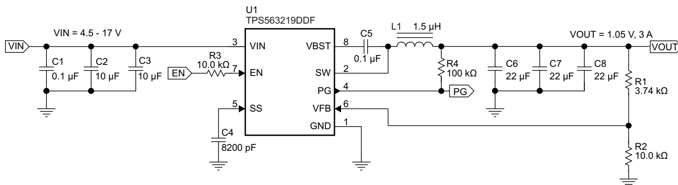
Figure 30. TPS563219 1.05V/3A Reference Design
