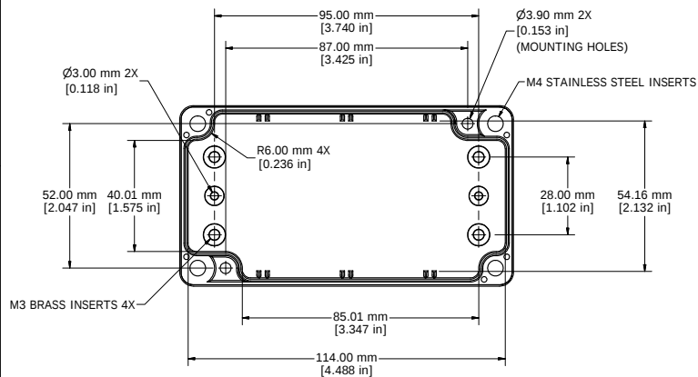
BOX - INSIDE
