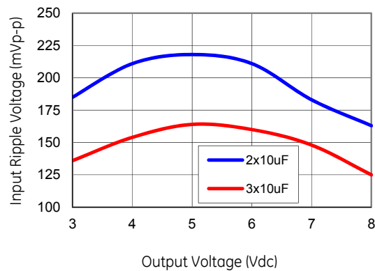
Figure 28. Input ripple voltage for various output voltages with 2x10 µF or 3x10 µF ceramic capacitors at the input (maximum load). Input voltage is 12V.
