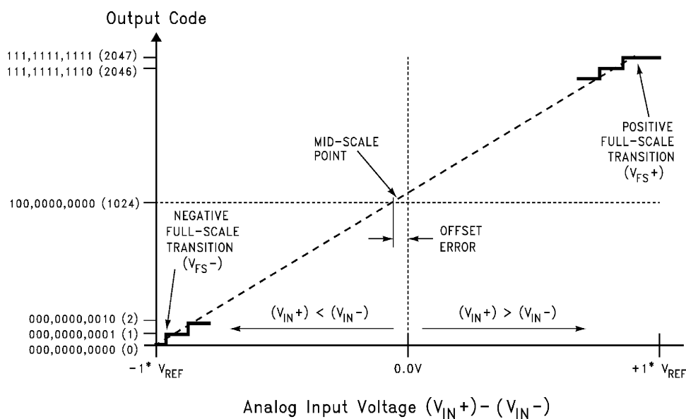
Figure 4. Transfer Characteristic
