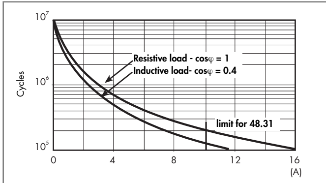
F 48 - Electrical life (AC) v contact current Types 48.31/61/81
