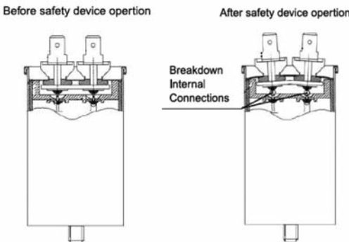
Fast-on terminals
