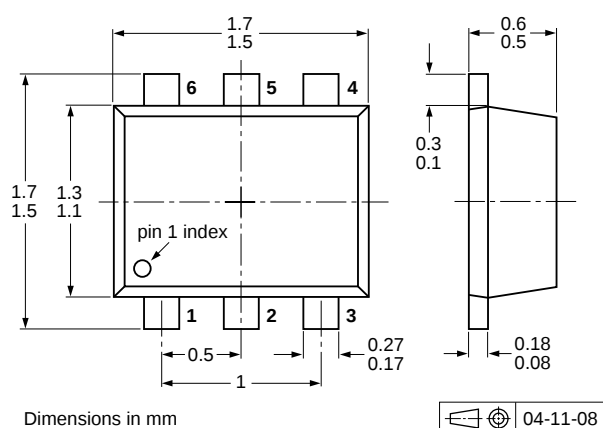
Fig 17. Package outline PEMD3 (SOT666)
