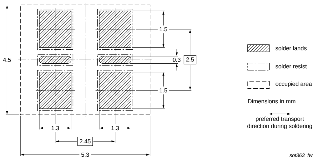
Fig 23. Wave soldering footprint PUMD3 (SOT363/SC-88)
