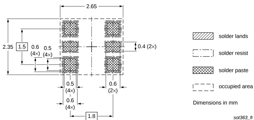
Fig 22. Reflow soldering footprint PUMD3 (SOT363/SC-88)
