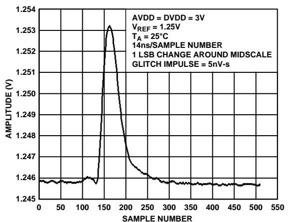
Figure 13. AD5381-3 Glitch Impulse
