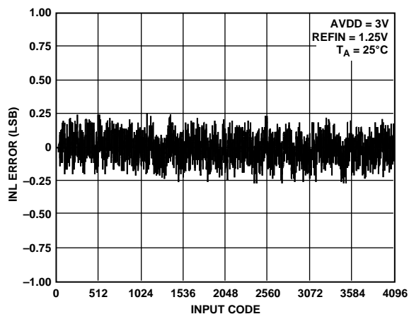
Figure 12. Typical AD5381-3 INL Plot
